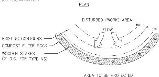
Figure 3. Compost Filter Sock - Type “B”
