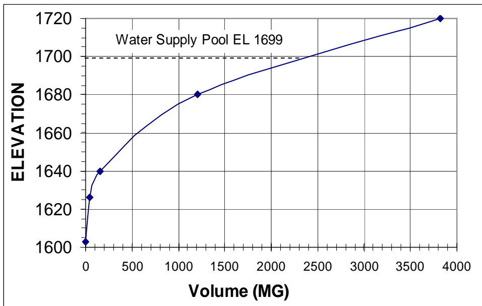
Figure 6 Stage-Storage Curve
